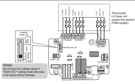
For no Power Contact Point signal Input
