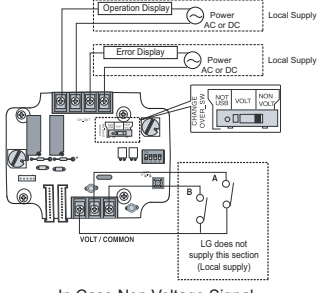
In Case Non Voltage Signal
