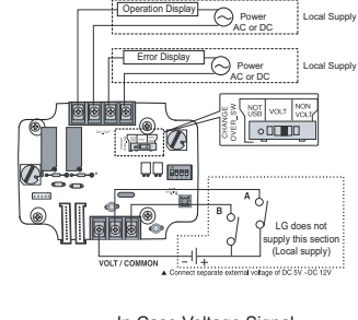
In Case Voltage Signal
